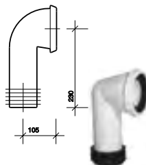
WC S connector WF1241WH
